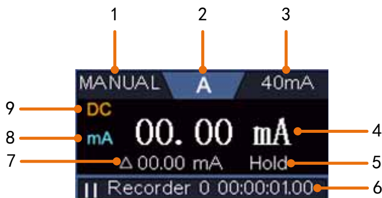
Figure 0-3 Multimeter Information Window
