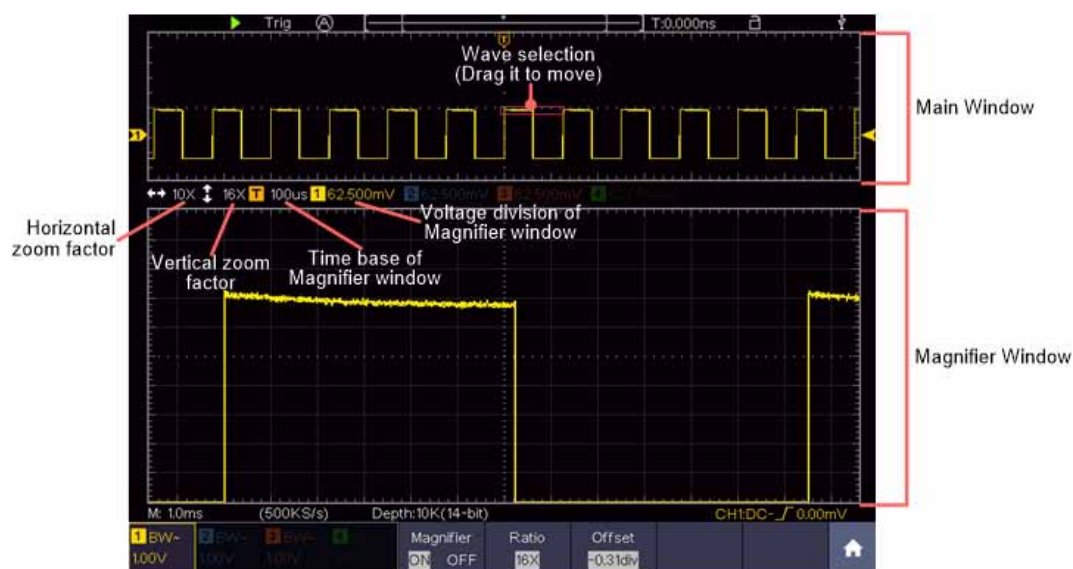
Figure 0-9 Magnifier Mode
