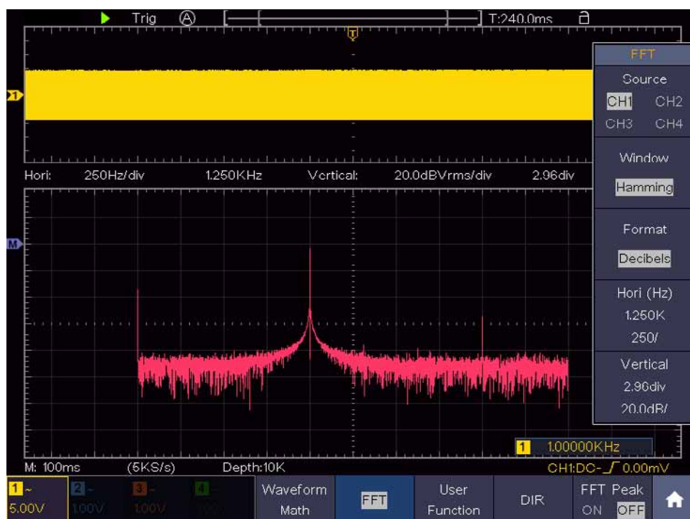
Figure 0-1 Hamming window
