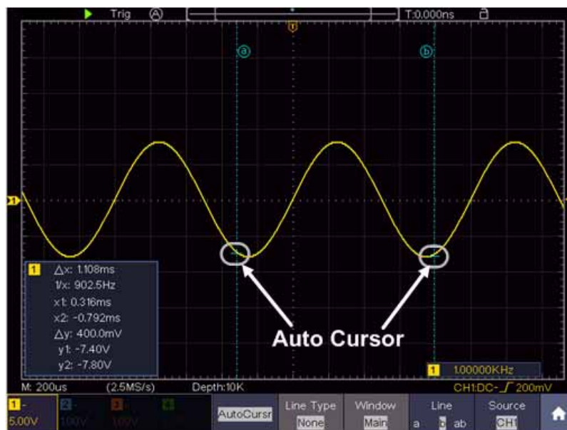
Figure 0-28 Auto Cursor
