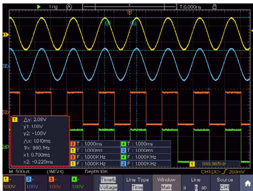
Figure 0-27 Time&Voltage Cursor Measurement
