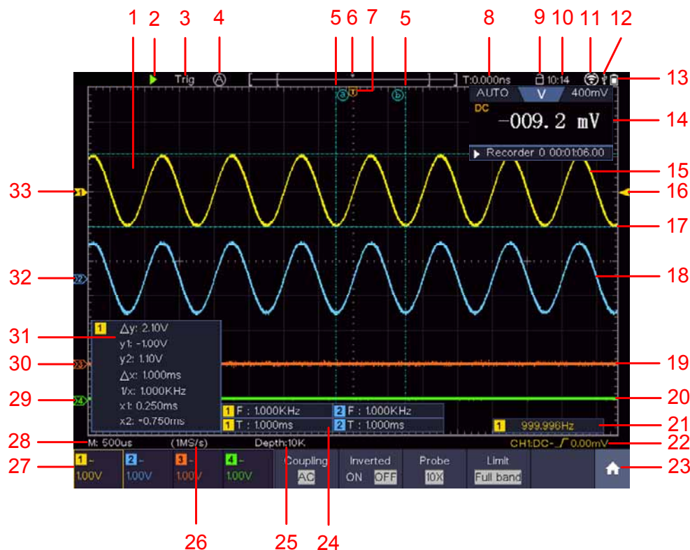
Figure 0-4 Illustrative Drawing of Display Interfaces
