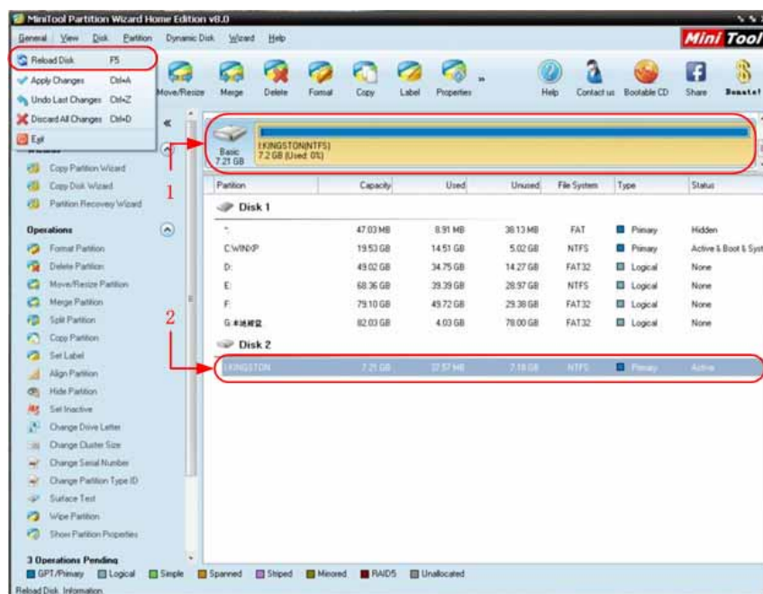
Figure 0-17: Reload Disk
