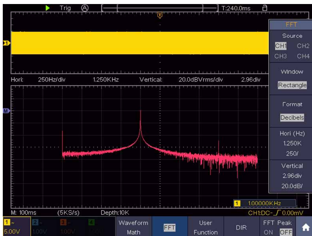
Figure 0-2 Rectangle window
