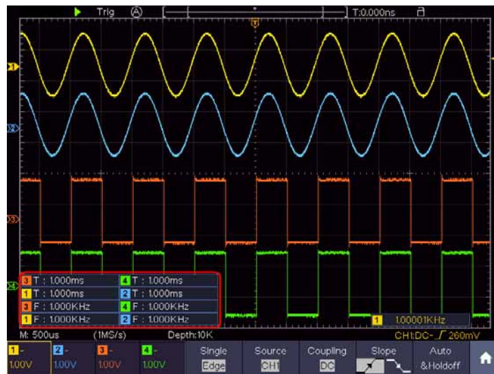
Figure 0-24 Automatic measurement
