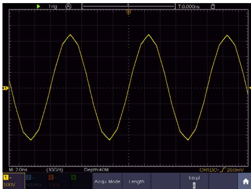
Figure 0-11 Linear interpolation
