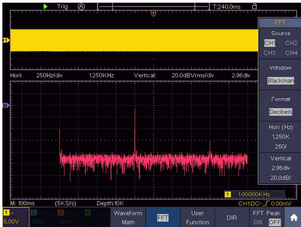
Figure 0-3 Blackman window
