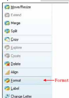
Figure 0-18: Choose format
