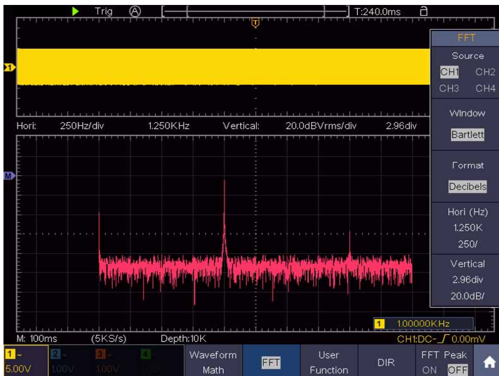
Figure 0-6 Bartlett window
