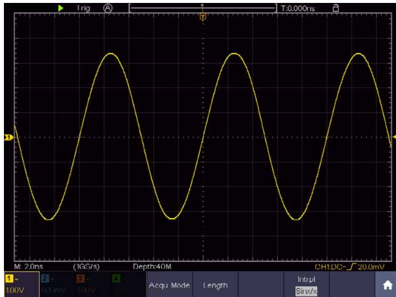
Figure 0-10 Sine(x)/x interpolation
