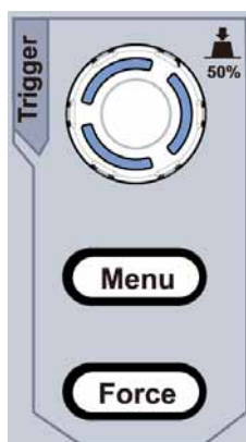
Figure 0-12 Trigger Control Zone
