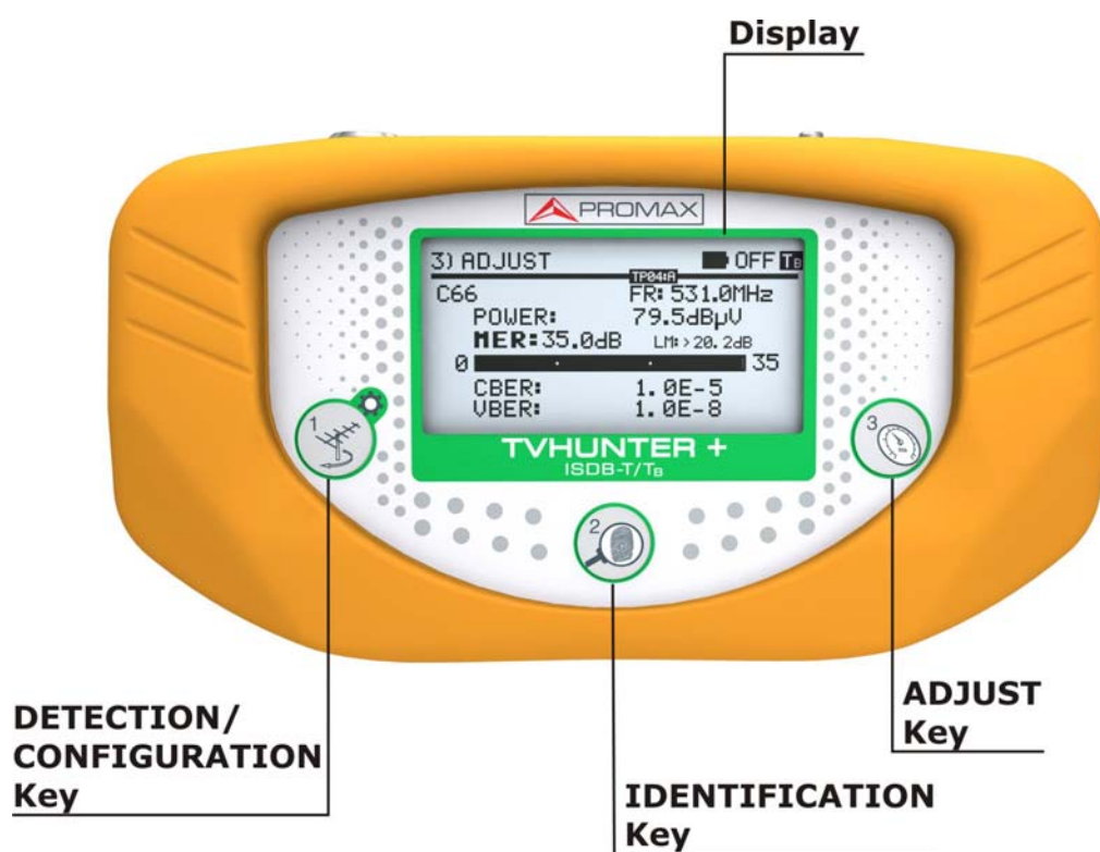
Figure 5. Front panel.
