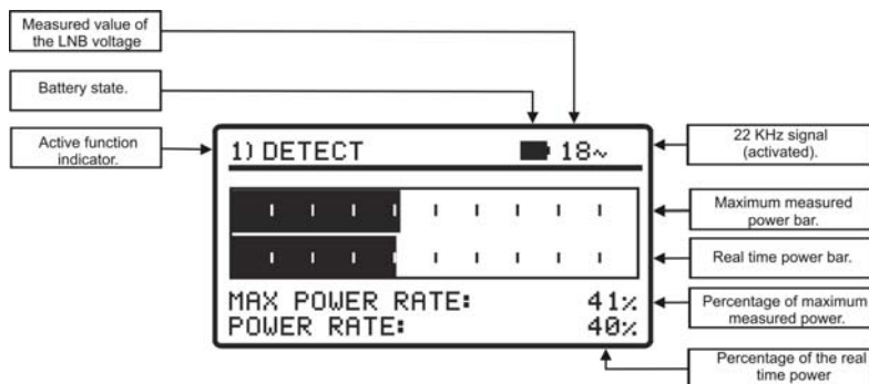
Figure 10.- DETECT function.
