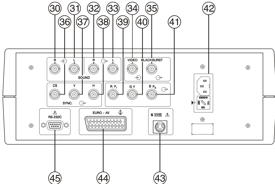
Figure 3.- Rear panel
