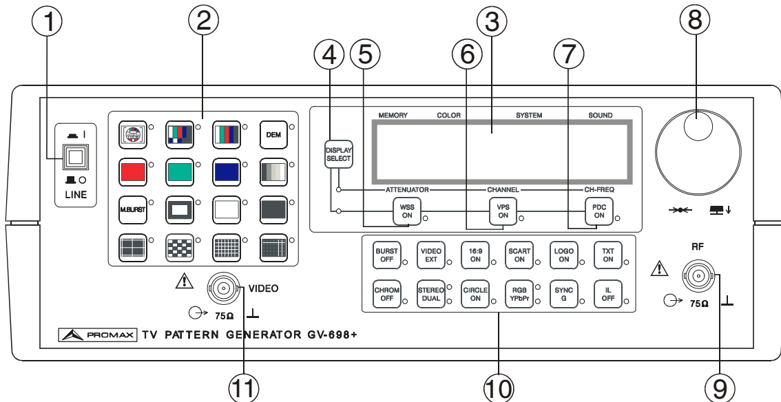
Figure 2.- Front panel
