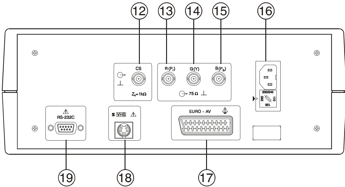
Figure 3.- Rear panel
