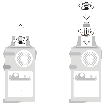
Figure 6.- Connecting external attenuator on RF input [30].
