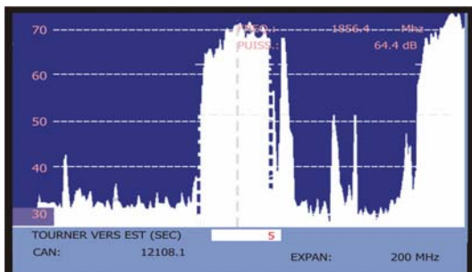
Figure 71.- Commandes DiSeqC: TOURNER VERS.
