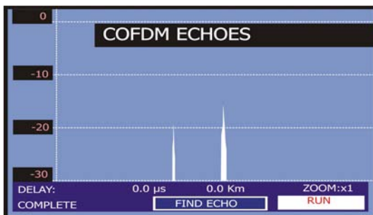
Figura 57.- ECHOES found.
