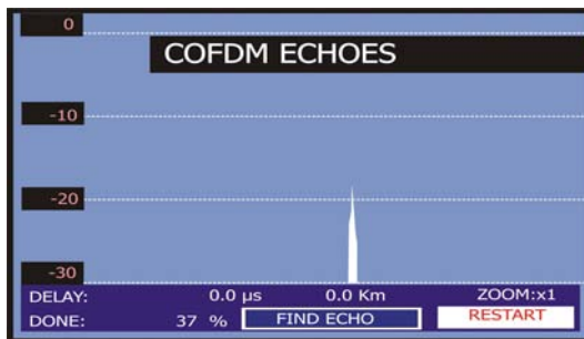
Figure 56.- Finding ECHOES.
