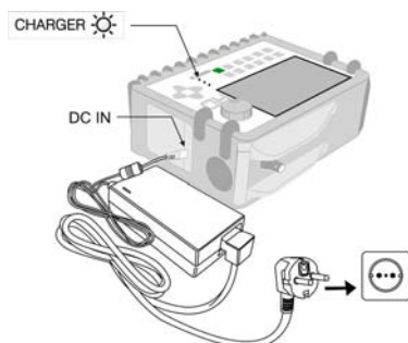
Figure 1.- Battery charging
