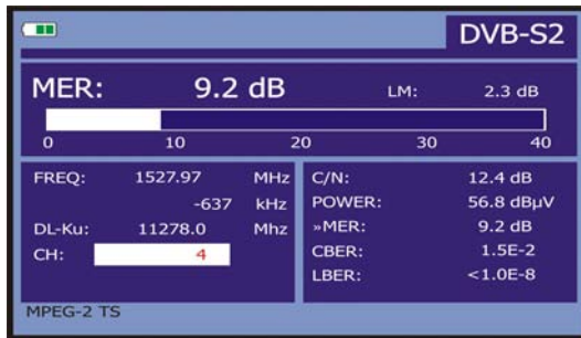
Figure 40.- DVB-S2 (QPSK/8PSK) signals MER measurement screen.
