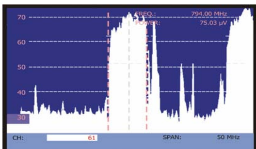
Figure 46.- Spectrum analyser mode.
