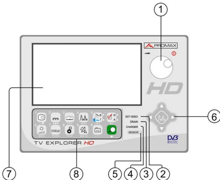
Figure 3.- Front panel.
