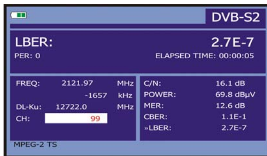
Figure 38.- DVB-S2 (QPSK/8PSK) signals LBER measurement screen.
