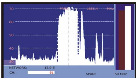
Figure 69.- Utility for antenna alignment.
