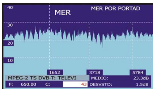
Figura 49.- Fonction MER by carrier.
