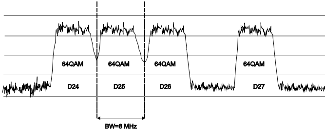
Figure 20.- Example of digital channels spectrum.
