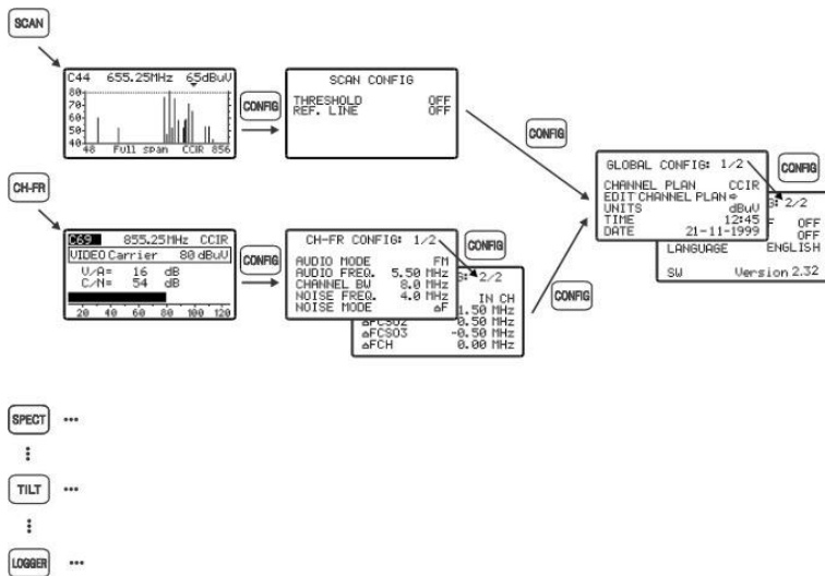
Figure 4.- Accessing the PROMAX-8 SE configuration menus.
