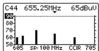
Figure 10.- SCAN mode, Ref. 90 dBuV.
