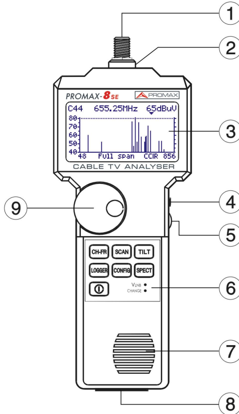
Figure 2.- Front panel.
