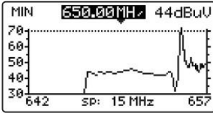
Figure 36.- MIN mode. First scan.
