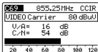
Figure 14.- V/A and C/N Level measurement
