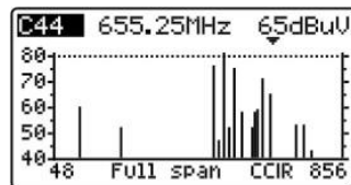
Figure 8.- SCAN mode, full span.
