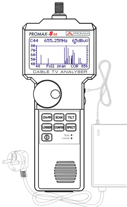
Figure 1.- PROMAX-8 SE and mains adapter connection.
