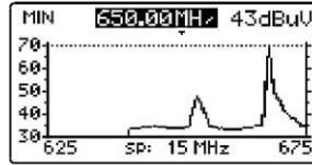
Figure 37.- After several scans.
