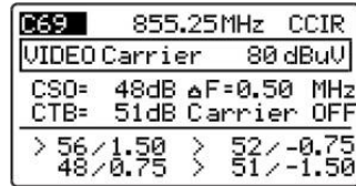
Figure 17.- CSO and CTB measurement.
