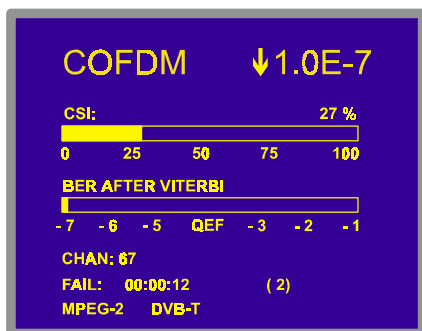
Figure 16.- Signalling two MPEG-2 signal cuts with a total length of 12 seconds.
