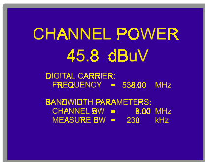
Figure 11.- Digital channel power measurement.
