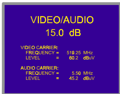
Figure 8.- Video/Audio rate measurement
