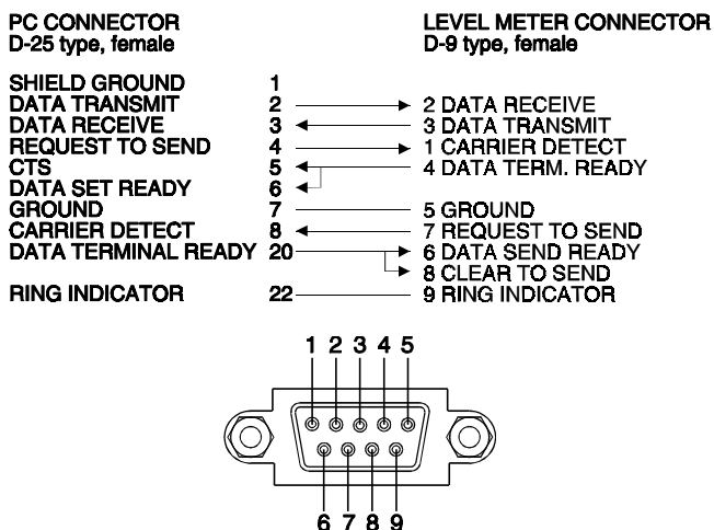
Figure 47.- Connector RS-232C PROLINK-4. Pins numbering.
