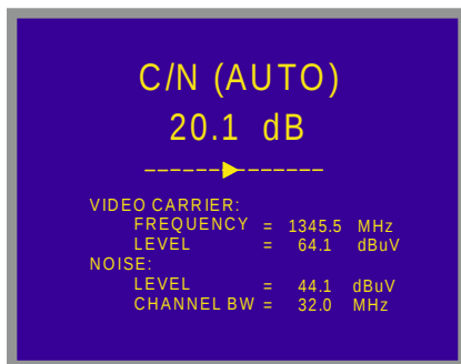
Figure 9.- Carrier-to-noise ratio measurement (Satellite band, analogue signal).
