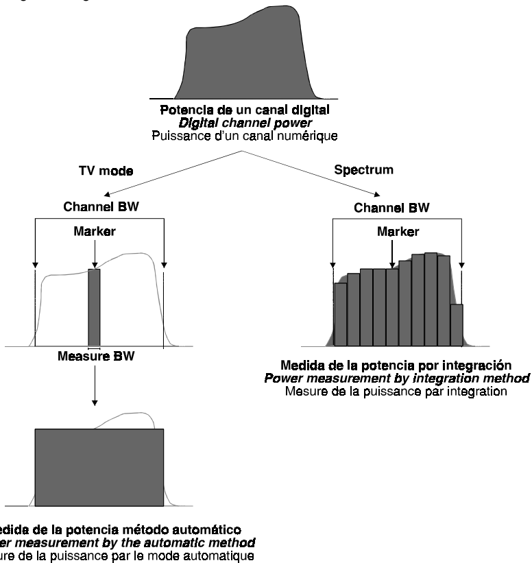
Figure 10.- Measuring digital power.
