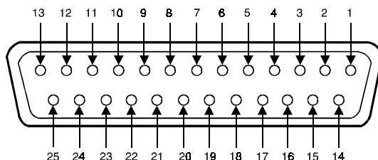
Figure 51.- Parallel Connector (LVDS D-25). External view.
