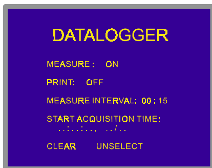
Figure 31.- Configuration of the DATALOGGER function
