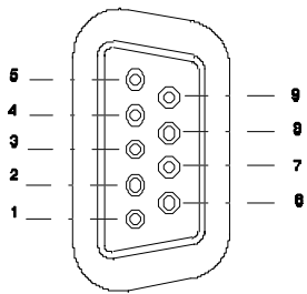
Figure 50.- RS-232C connector. External view.
