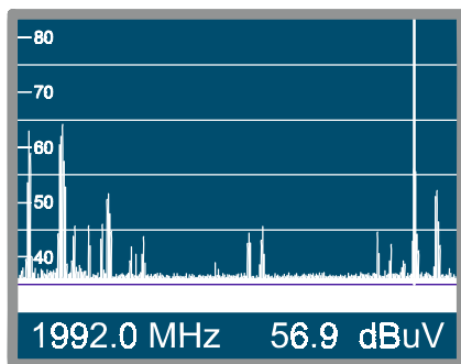
Figure 39.- Spectrum Analyser mode.
