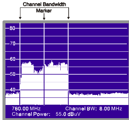
Figure 43.- Channel power measurement in Spectrum Mode.
