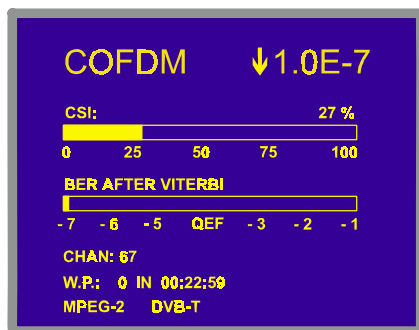
Figure 14.- BER measuring screen for COFDM-modulated signals
