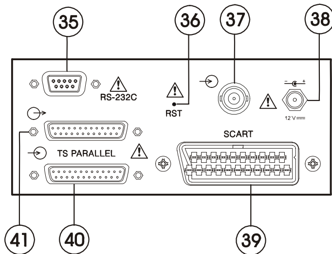
Figure 3.- Side panel connections.
