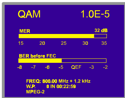
Figure 12.- BER measuring screen for QAM-modulated signals.
